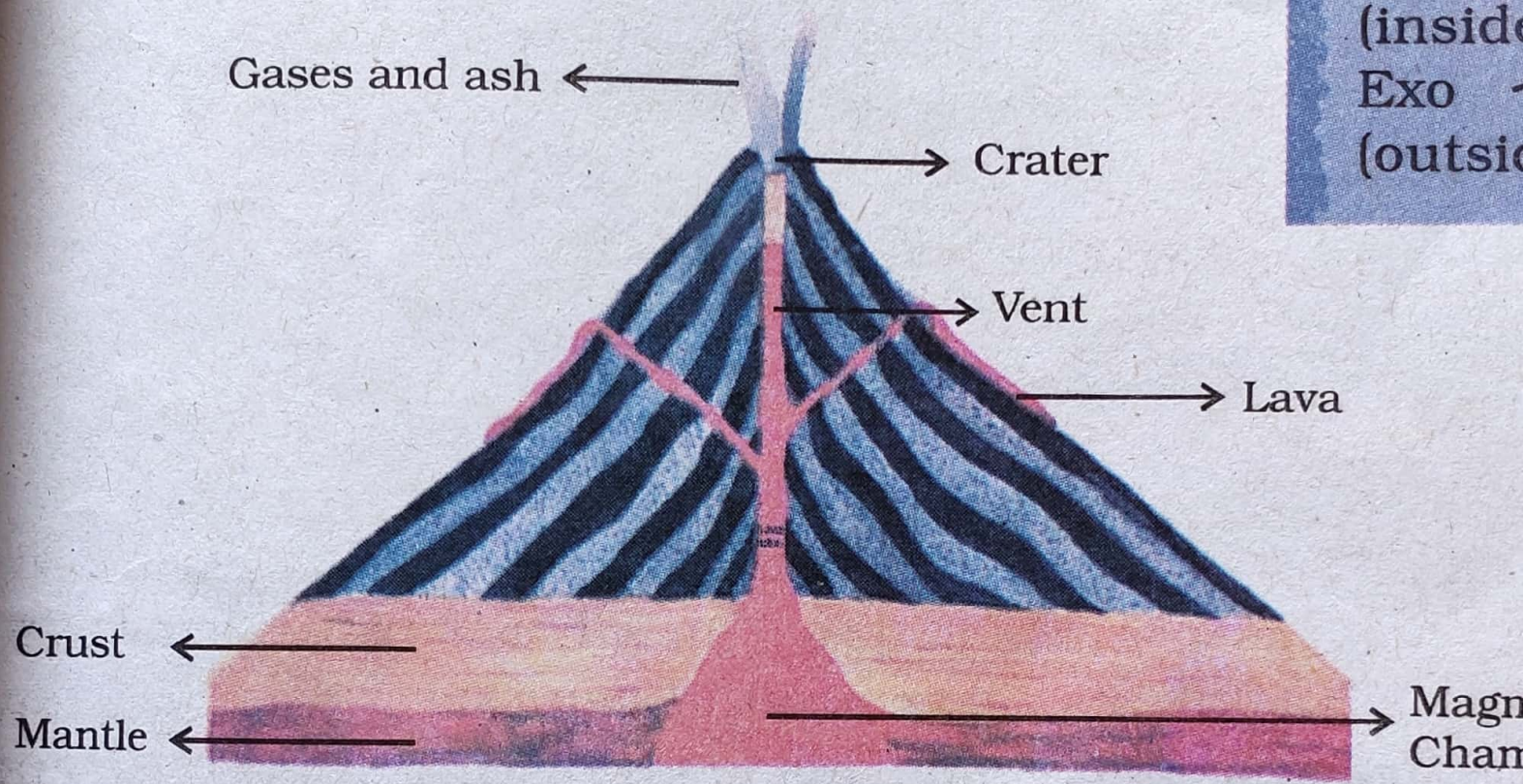
Fig. 3.2: A Volcano
